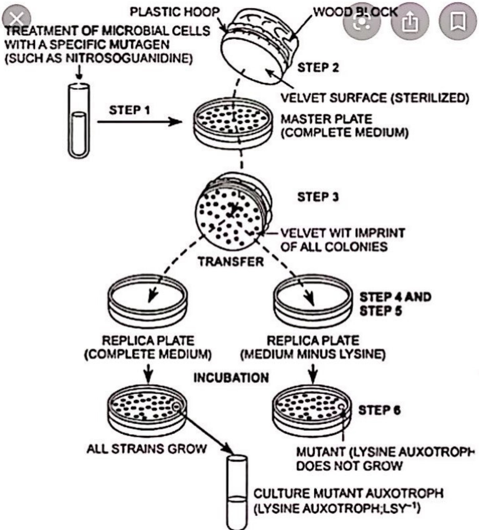
FIG. 29.13. Replica plating technique used for selection of nutritional mutants.
